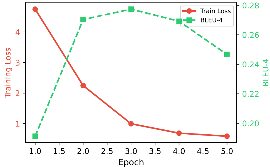
Low-LR FT
