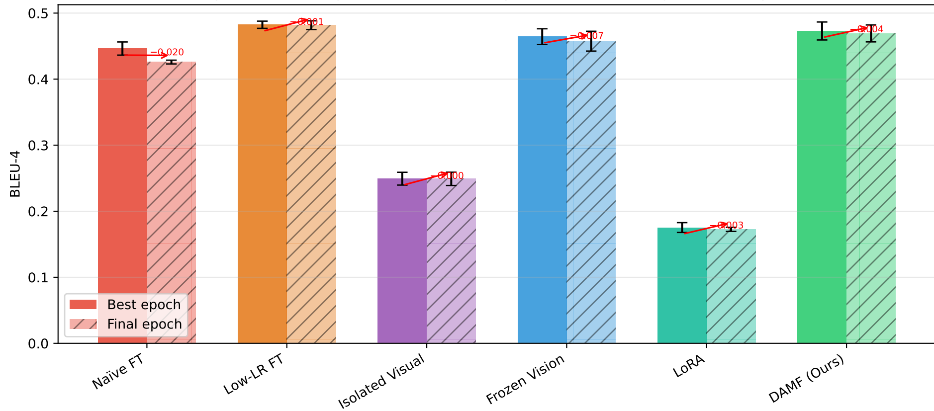
RSICD — Best vs Final Epoch BLEU-4 (Stability) Compare to UICD Fig 3 — RSICD shift may be milder, less degradation expected
