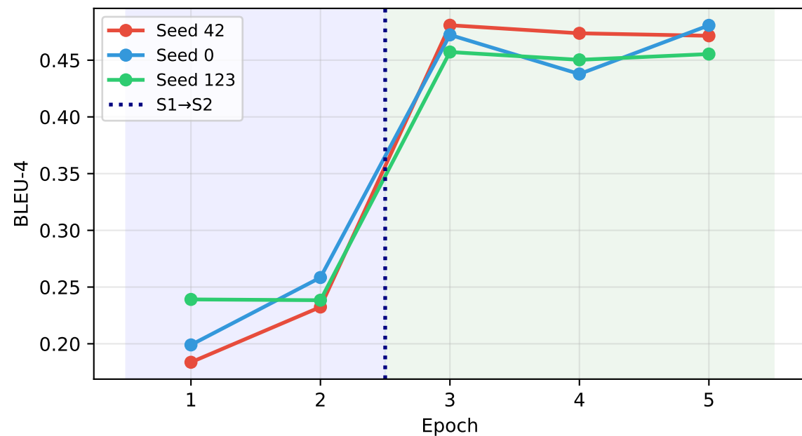
DAMF RSICD — BLEU-4 across 3 Seeds
