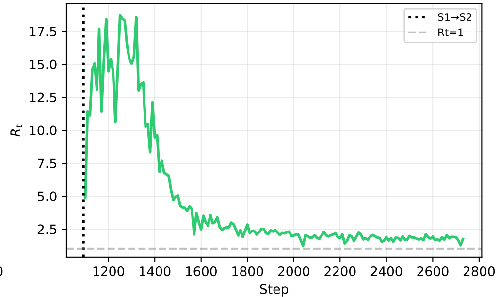
DAMF RSICD — Seed 123
