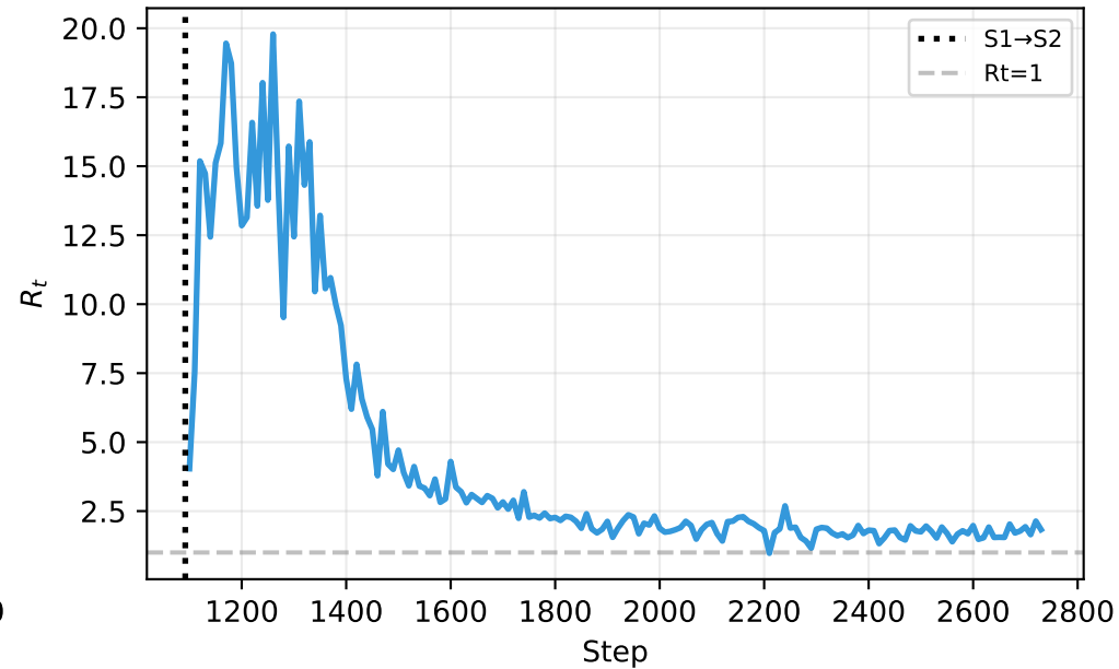
DAMF RSICD — Seed 0
