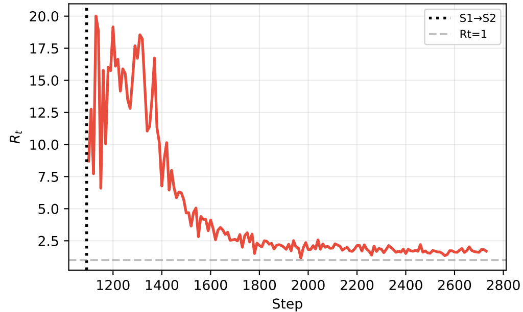
DAMF RSICD — Seed 42
