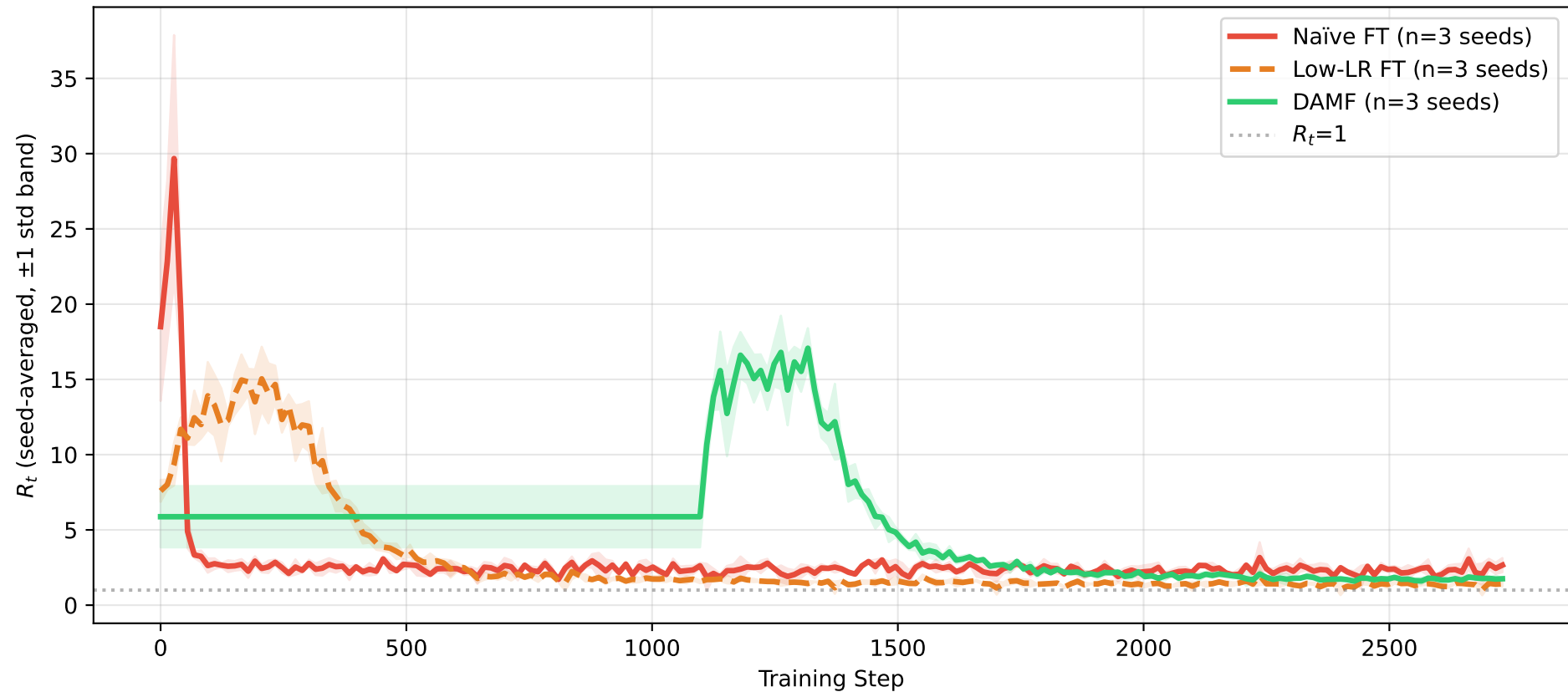
RSICD — Gradient Imbalance: Naïve FT vs Low-LR FT vs DAMF Seed-averaged across all available seeds
