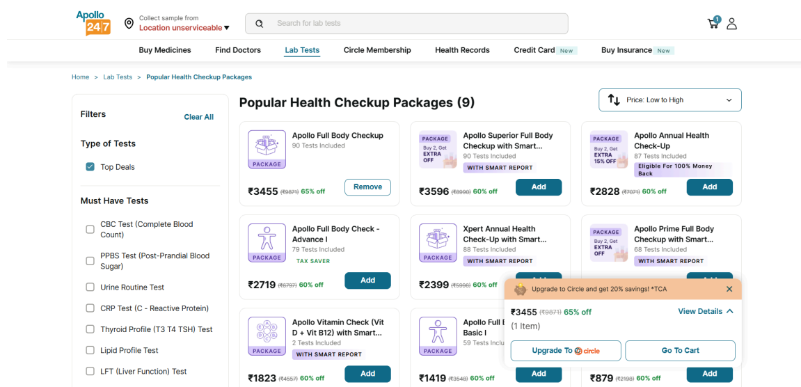
Fig 10: 09_package_added
