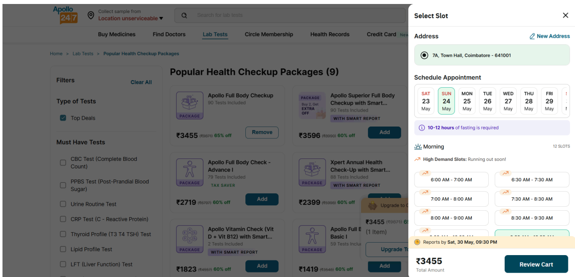
Fig 14: 13_schedule_selected
