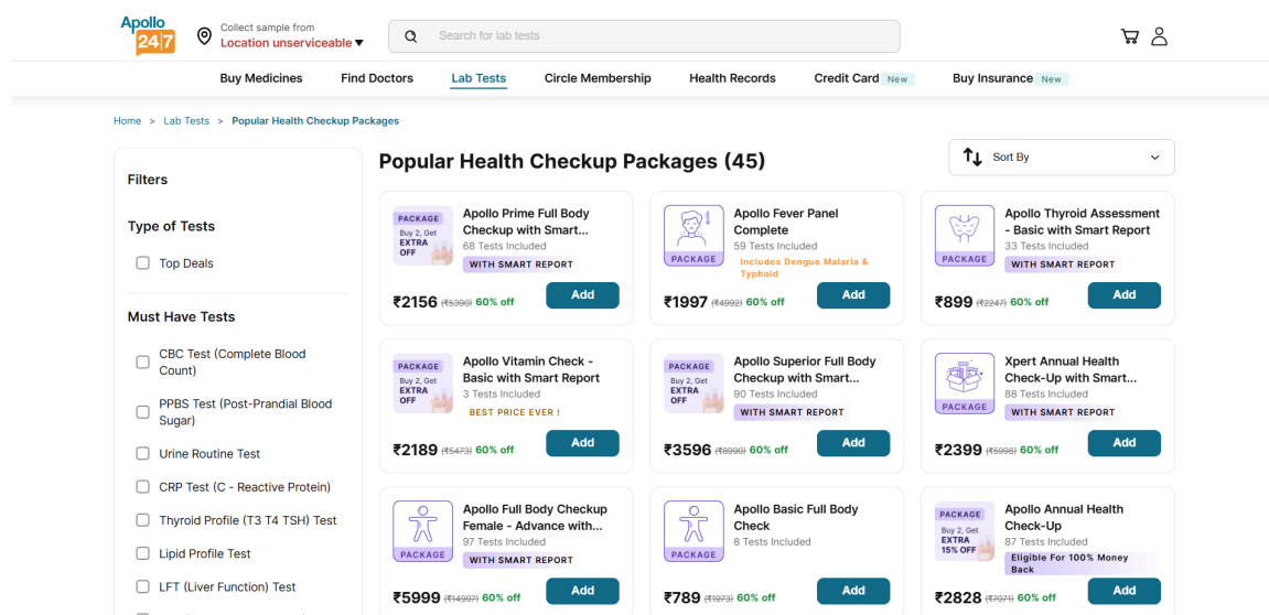
Fig 6: 06_popular_packages_listing
