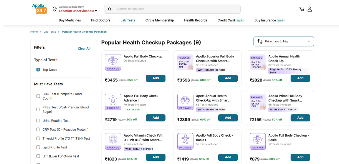
Fig 9: 08_sort_low_to_high
