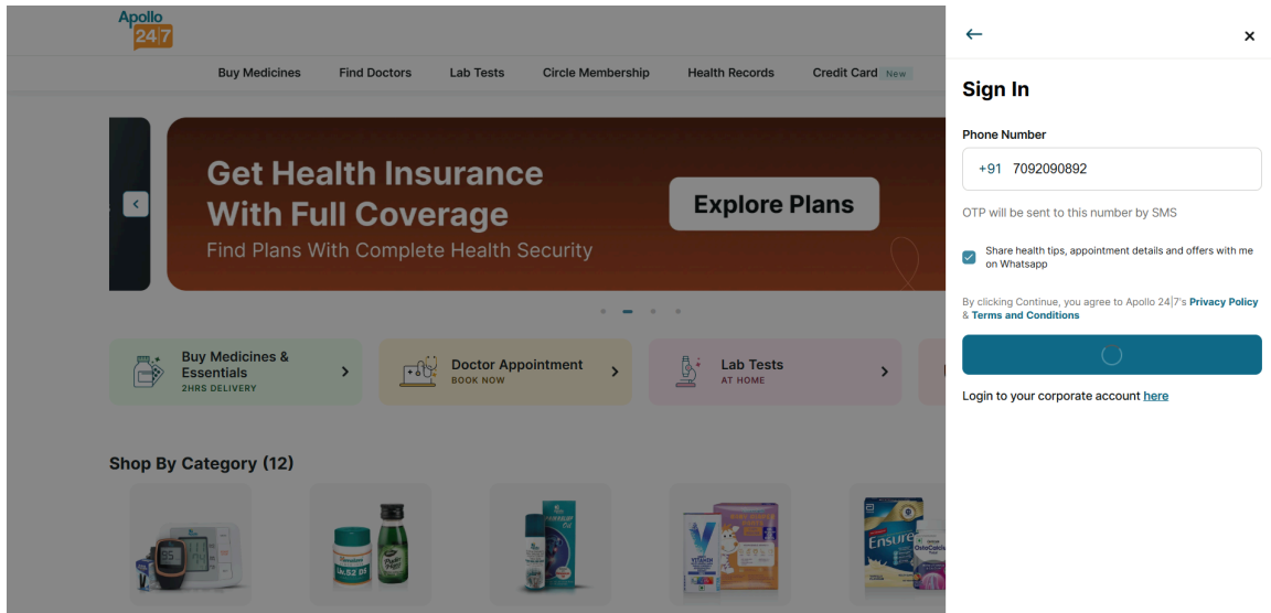
Fig 3: 03_otp_screen
