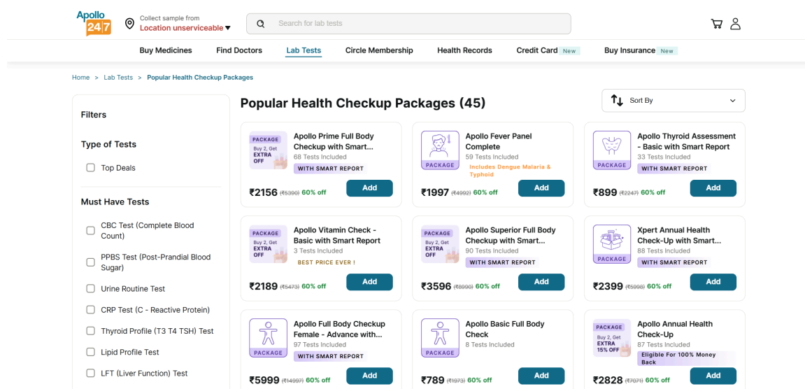
Fig 6: 06_popular_packages_listing
