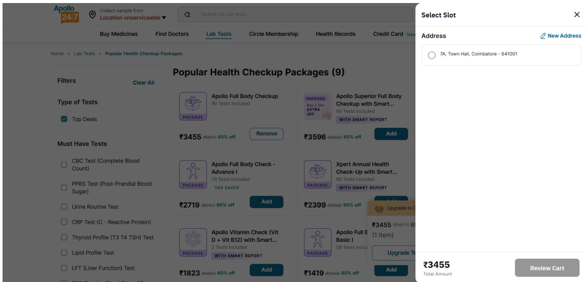
Fig 12: 11_patient_selected
