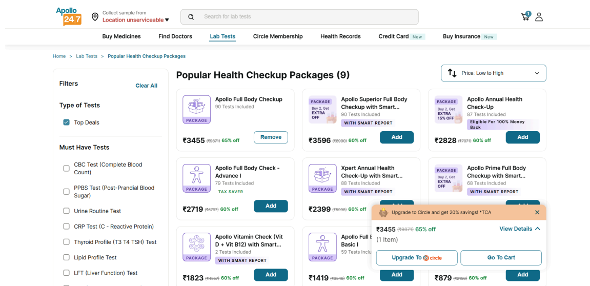
Fig 10: 09_package_added
