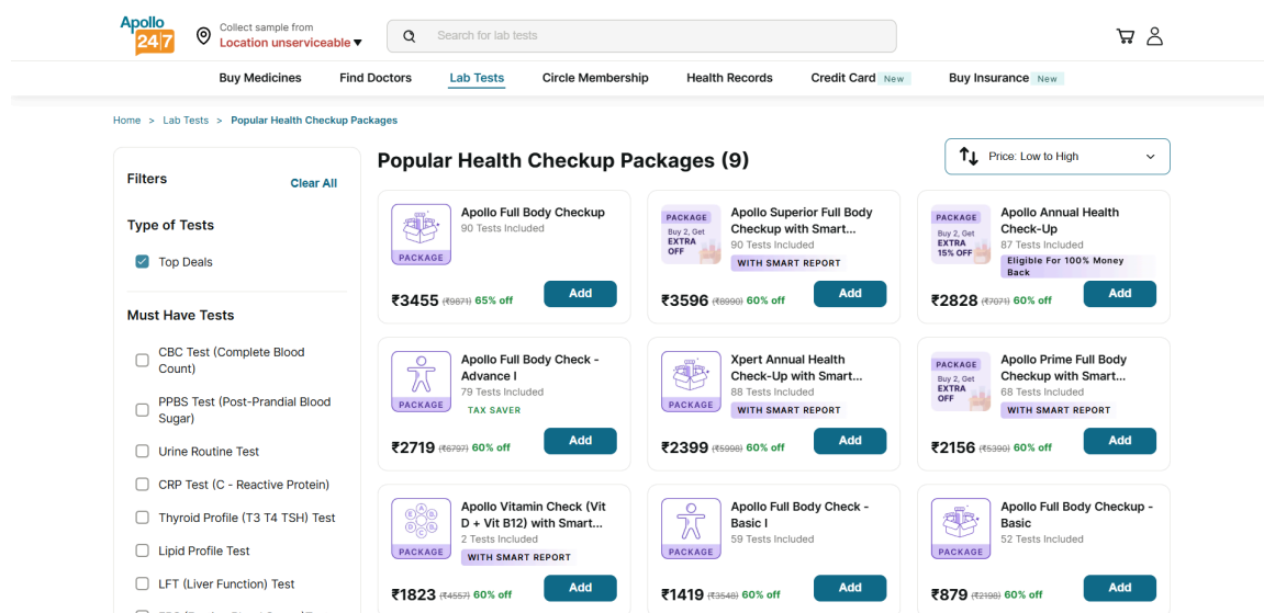
Fig 9: 08_sort_low_to_high
