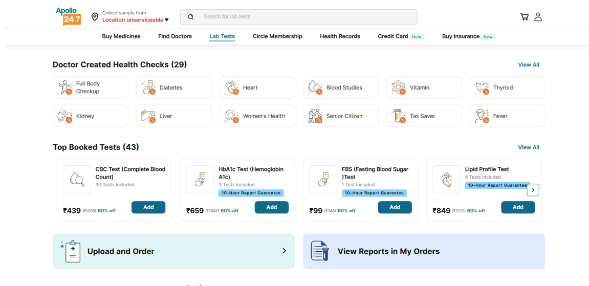
Fig 5: 05_lab_tests_page
