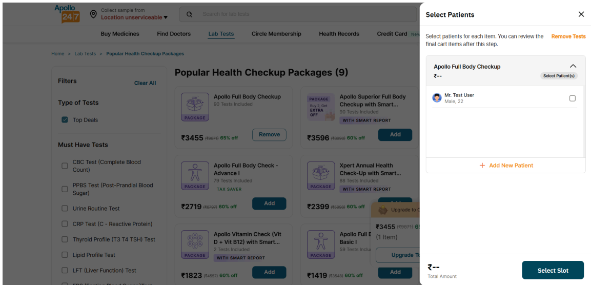
Fig 11: 10_cart_popup
