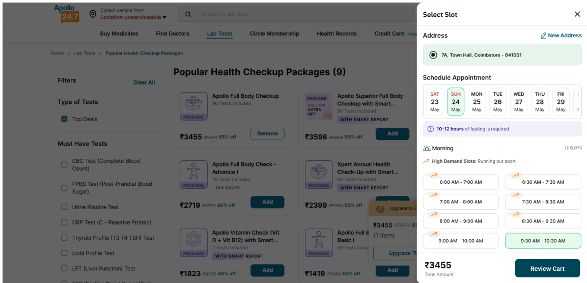
Fig 13: 12_address_selected
