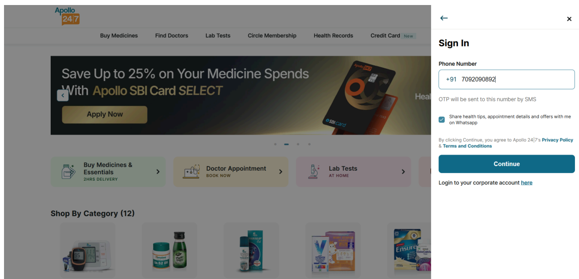
Fig 2: 02_mobile_entered
