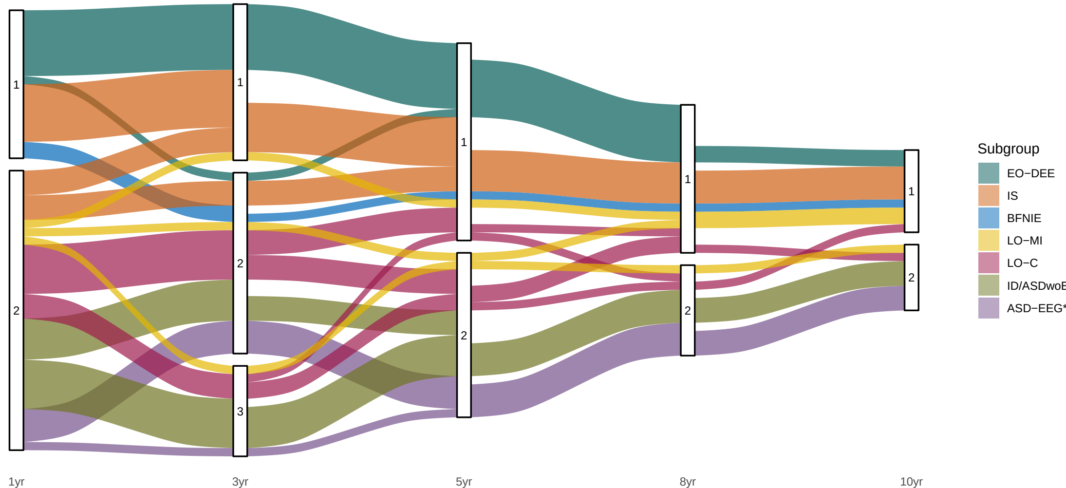
Change in Cluster Membership Across Age Cut-offs
