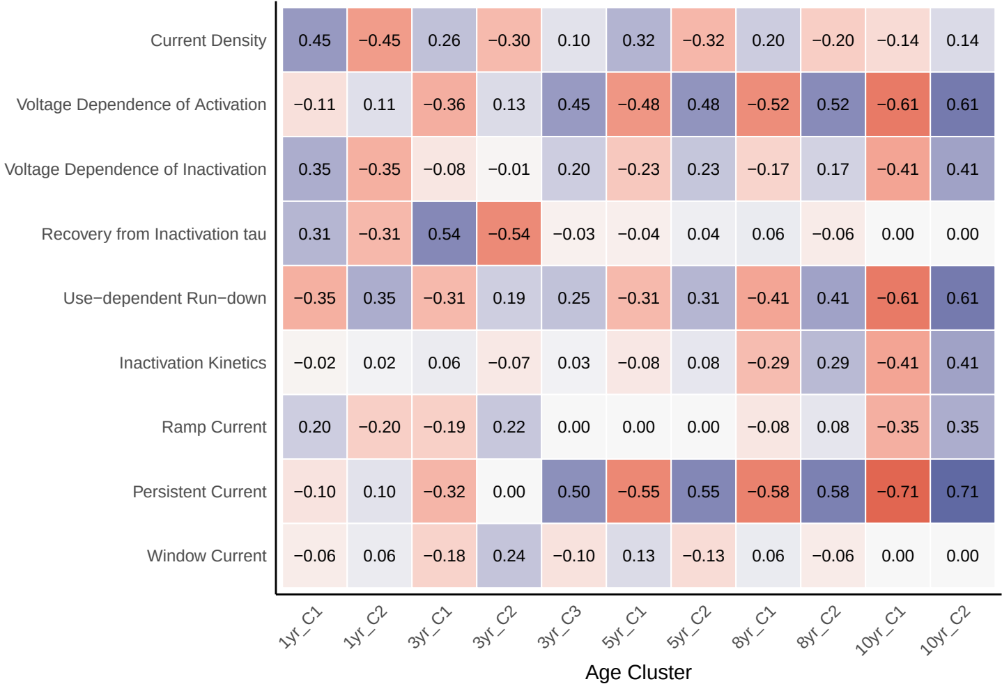
Adult: Cluster vs. Biophysics Correlation
