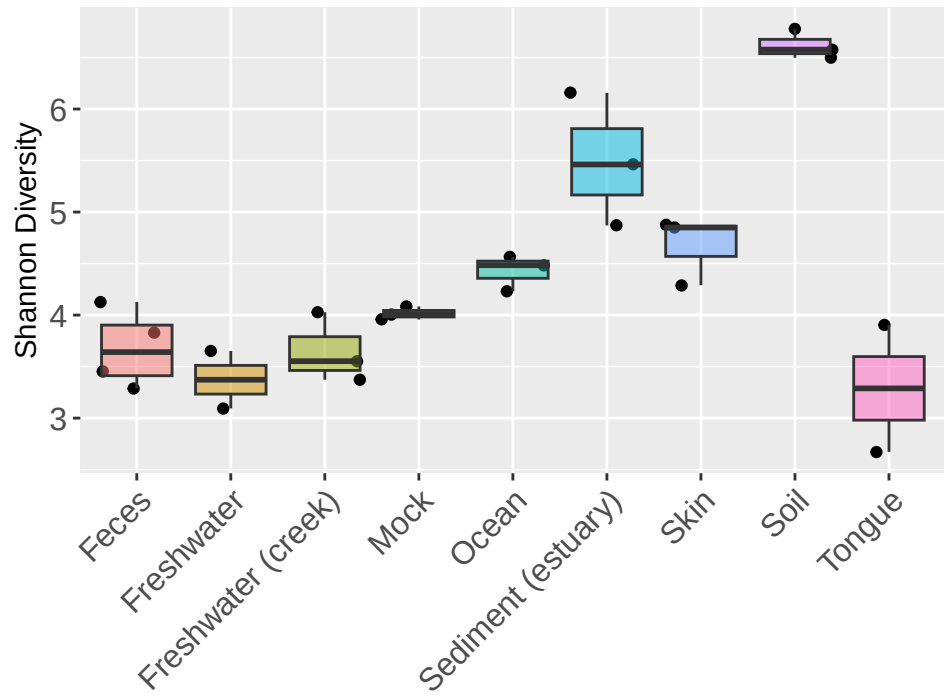
Shannon Diversity by Sample Type
