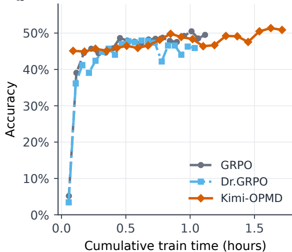
b Accuracy per recorded training time
