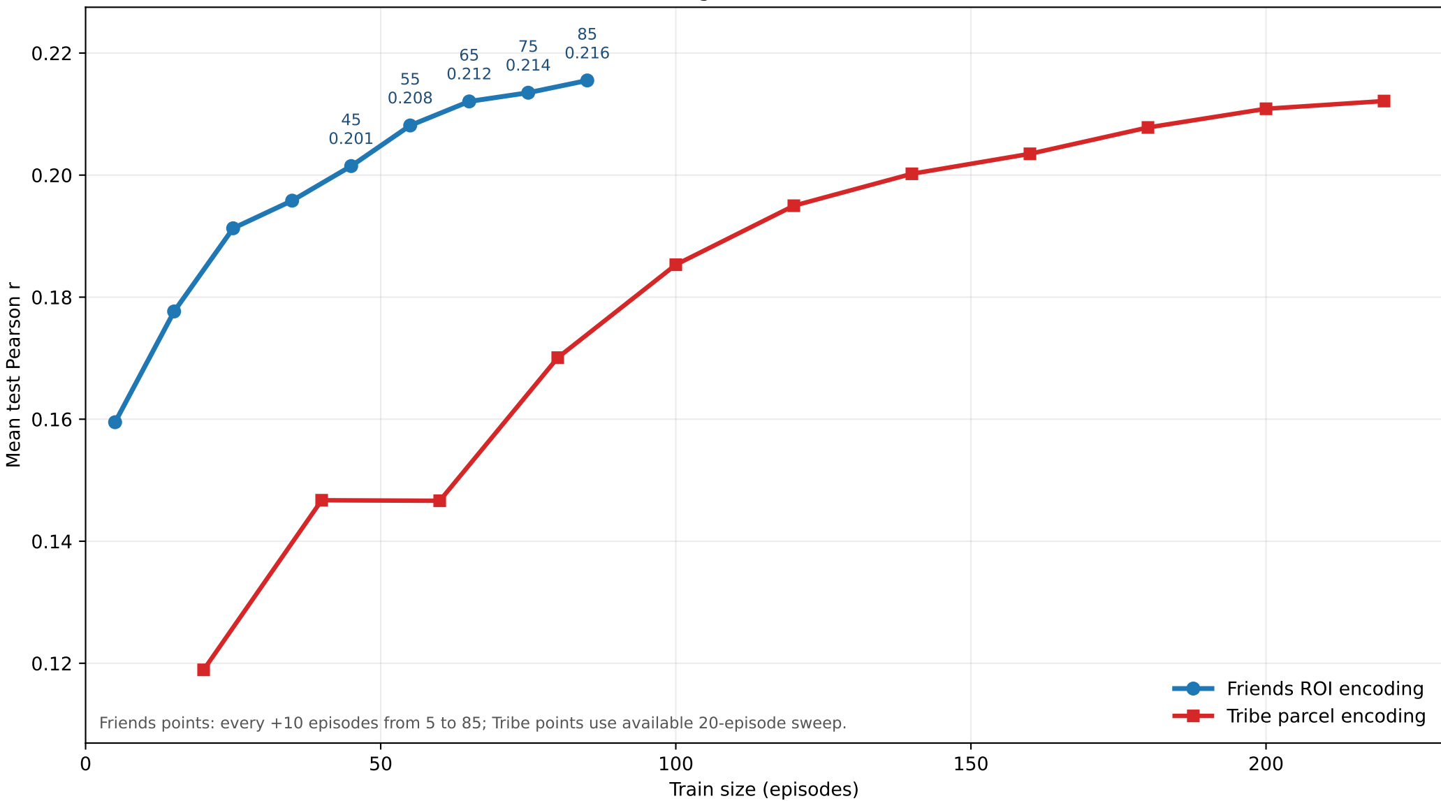
Train Size vs Encoding Performance: Friends and Tribe
