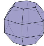
4 Droxtal scale=1 convex
