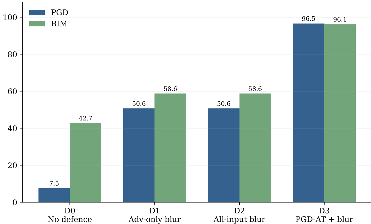
Robust accuracy at \varepsilon = 4/255 (%)
