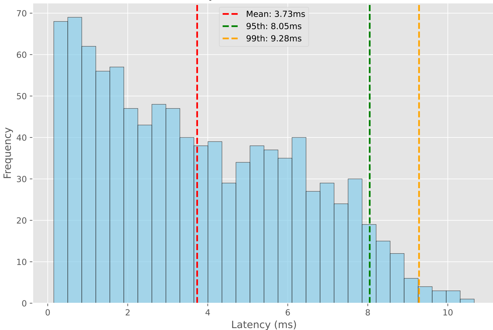
End-to-End Latency Distribution (Load: 1000 iterations)
