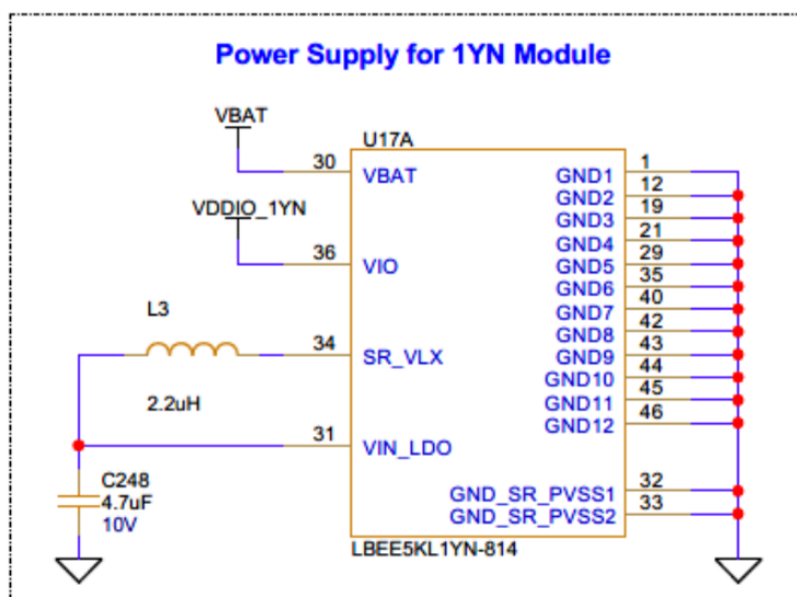
1YN module power supply schematic
