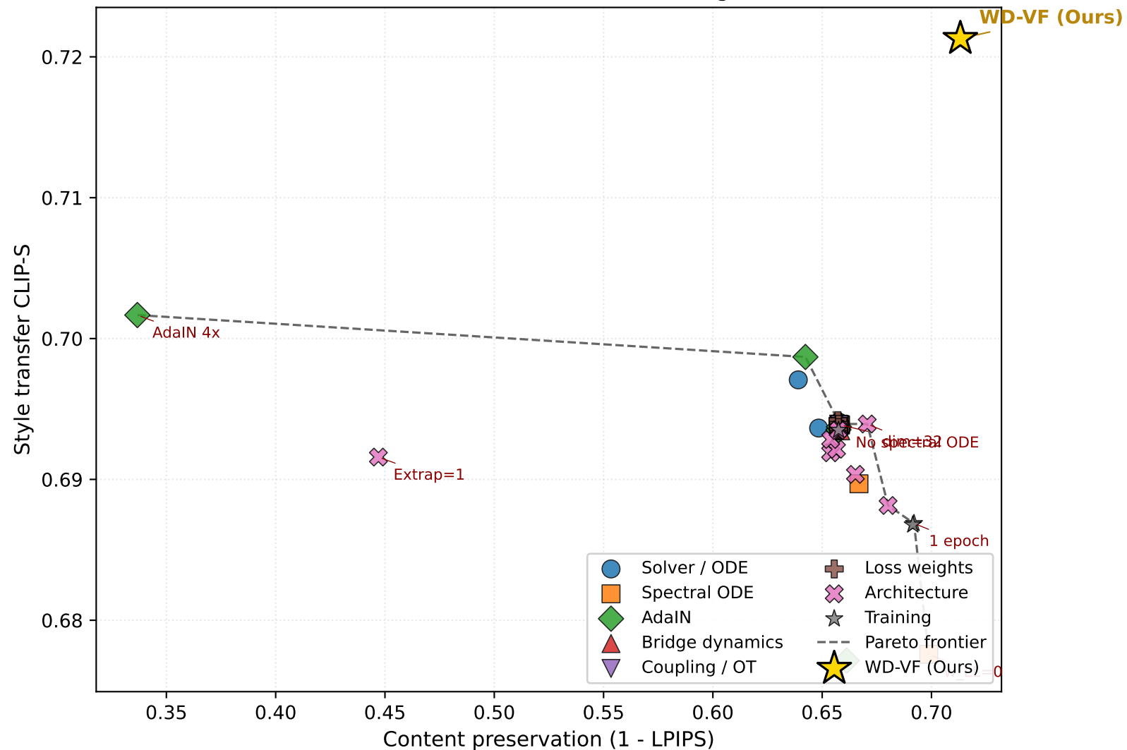
512-resolution ablation (48 configs)
