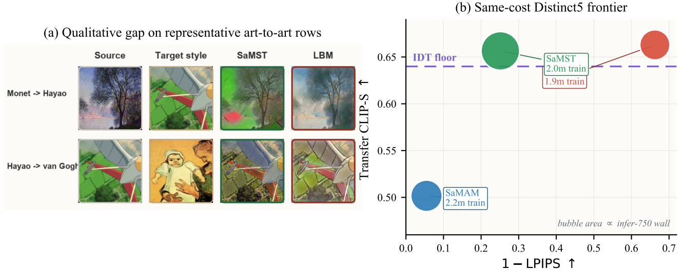
Figure 1: Teaser summary of the paper’s two practical claims. In (a), two representative art-to-art rows from the historical standard benchmark show the qualitative failure mode of the closest efficient baseline: SaMST can push stronger raw texture, but it does so with muddy grain, color spill, and broken local edges, whereas LBM keeps cleaner target-style movement on the same rows. In (b), the same-cost Distinct5-512 frontier quantifies the matched-budget stress test: higher and further right is better, the dashed line marks the transfer-only IDT floor, and bubble area denotes infer-750 wall time. The LBM bubble corresponds to the explicit step-350 packet used for the matched-budget comparison; the earlier LBM frontier points near 1.2 minutes are discussed later. Under matched roughly two-minute training budgets, LBM still occupies the favorable region, same-cost SaMST stays only slightly above IDT at much larger displacement, and same-cost SaMAM remains below IDT.
