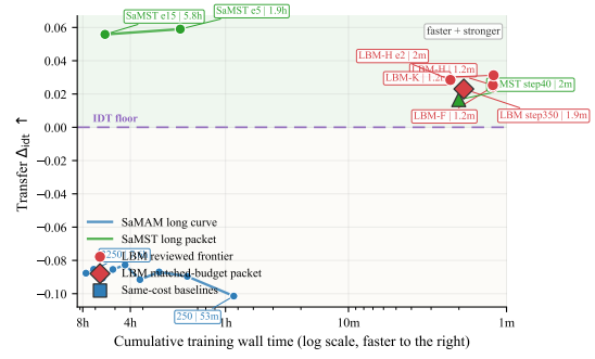
Figure 5: Evidence-closed Distinct5 timing records plotted as transfer-only \Delta_{idt} against cumulative training wall time under the reproduced full 5 \times 5 / 750 -output protocol. The horizontal axis is log-scaled and inverted so faster adaptation appears to the right. LBM is shown in two roles: the retained reviewed frontier points around 1.2 minutes and the later step-350 matched-budget packet used on page 1. SaMAM is shown both as the exact same-cost packet and as bounded pre-2250 timing records with the active manuscript boundary fixed at the trusted 2250 checkpoint; SaMST is shown both as the exact same-cost packet and as the longer retained operating point. The plot therefore preserves the calibration behind the page-1 summary rather than serving as a closed normalized time-to-parity claim.
