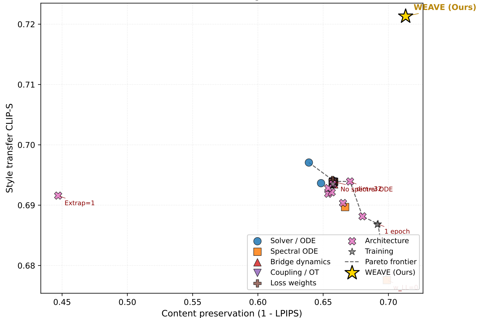
512-resolution ablation (43 configs, AdaIN axis omitted)
