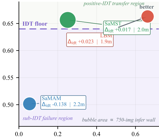
(b) Same-cost Distinct5 operating points
