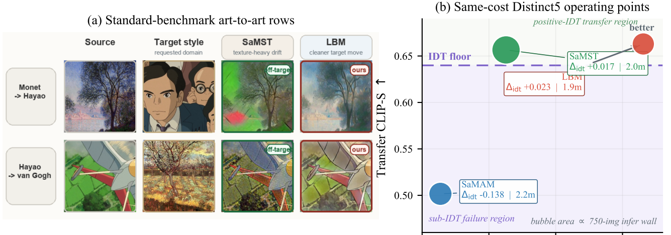
Figure 1: Page-1 teaser. Left: two art-to-art rows from the historical standard benchmark. SaMST drifts toward generic art-domain texture, whereas LBM moves more cleanly toward the requested target domain. Right: transfer CLIP-S versus 1 - \text{LPIPS} under matched roughly two-minute Distinct5-512 budgets. LBM lands in the favorable upper-right positive-IDT region; same-cost SaMST stays only slightly above the IDT floor at much larger displacement, and same-cost SaMAM remains below IDT. Bubble area denotes 750-image inference wall time.
