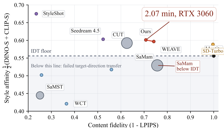
Figure 1: IDT-calibrated comparison on Distinct5-WikiArt. Left: style affinity \frac{1}{2}(\text{DINO-S} + \text{CLIP-S}) versus 1 - \text{LPIPS} , with bubble area encoding training time. The red points mark two WEAVE operating points. Square markers denote training-free diffusion editors (StyleAligned). The dashed line marks the IDT floor (0.556); methods below it have not moved in the requested direction. Right: target-pooled ArtFID on the same benchmark, with numbers inside the bars indicating training or response time.
