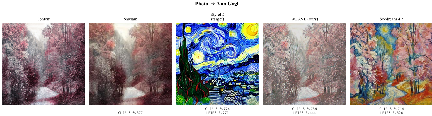
Figure 3: Qualitative comparison on Photo \Rightarrow Van Gogh (Photo2Art 256). Left to right: source (no-op), SaMam (near-identity), StyleID (high style), WEAVE (ours), Seedream 4.5 (commercial ref). WEAVE and Seedream 4.5 both move in the target direction while keeping the subject recognizable.
