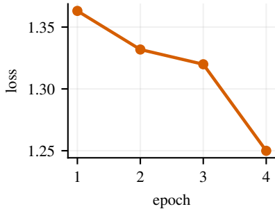
Training loss
