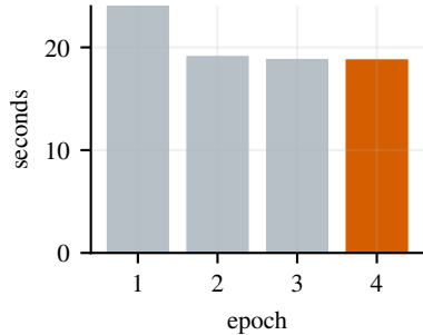
Epoch time
