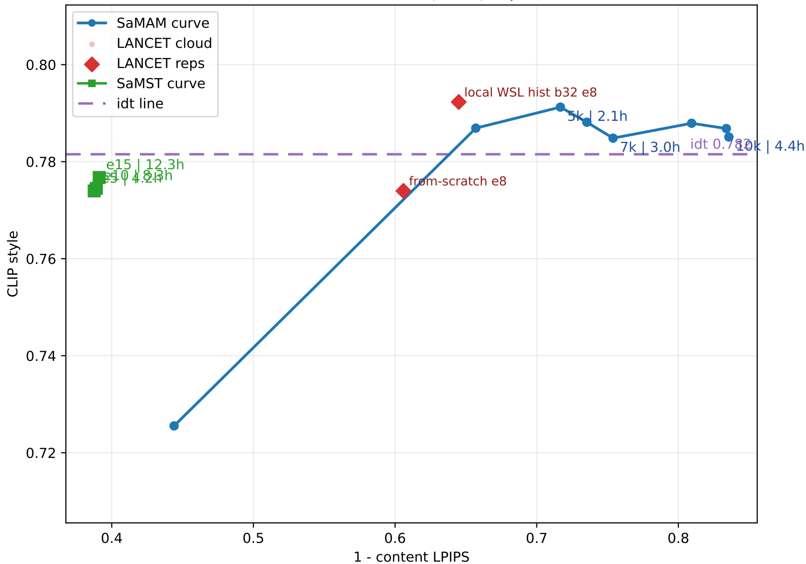
WikiArt512 / 3600 per style | full
