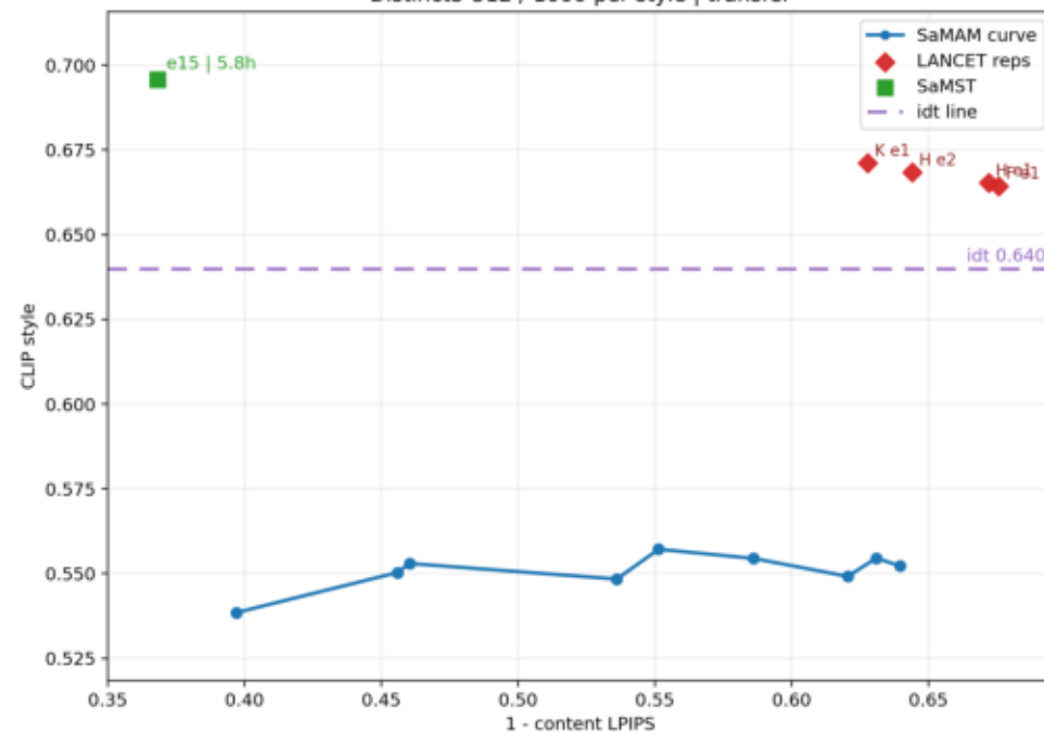
Distinct5-512 / 1000 per style | transfer
