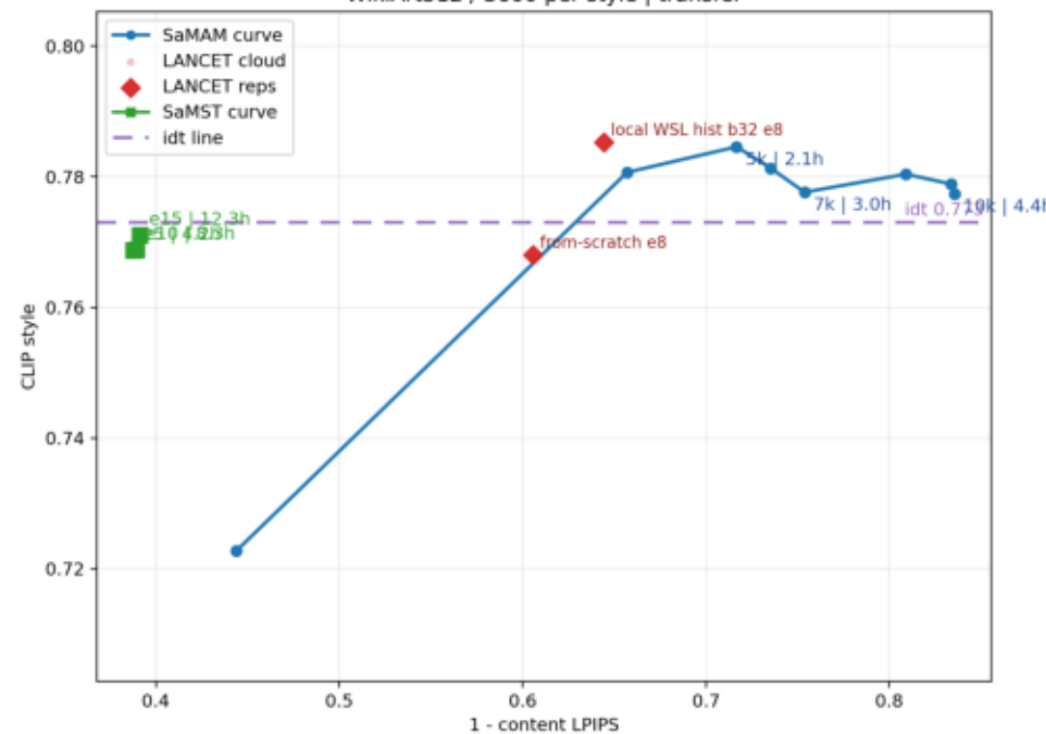
WikiArt512 / 3600 per style | transfer
