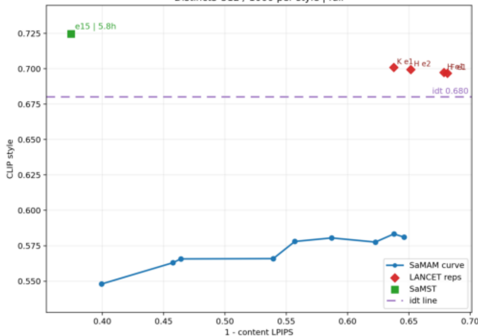
Distinct5-512 / 1000 per style | full
