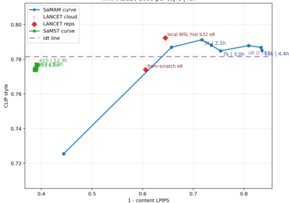
WikiArt512 / 3600 per style | full
