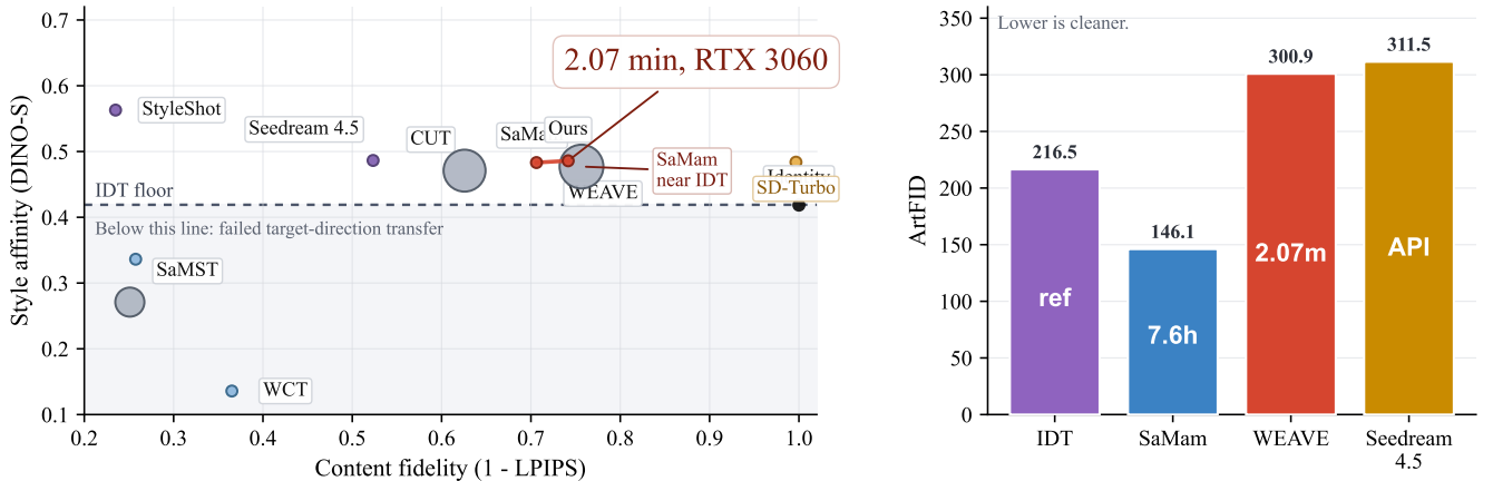
Figure 1: IDT-calibrated comparison on Distinct5-WikiArt. Left: DINO-S versus 1 - \text{LPIPS} , with bubble area encoding training time. The red points mark two WEAVE operating points. Square markers denote training-free diffusion editors (StyleAligned). The dashed line marks the IDT floor (0.419); methods below it have not moved in the requested direction. Right: target-pooled ArtFID on the same benchmark, with numbers inside the bars indicating training or response time.
