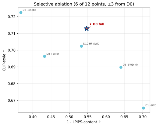
Figure 4: Destructive ablations. Removing SA-SWD improves content but weakens style, while removing kinetic regularization increases style at the cost of severe content degradation.
