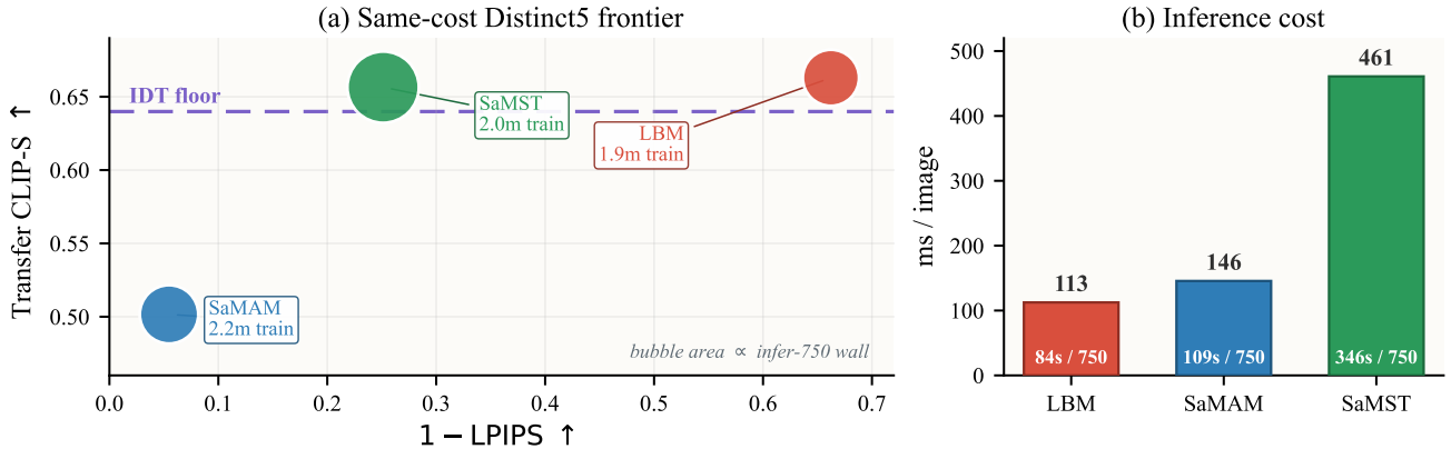
Figure 1: IDT-calibrated same-cost Distinct5-512 summary under the shared full 5 \times 5 / 750 -output packet. In (a), higher and further right is better: transfer CLIP-S is plotted against 1 - \text{LPIPS} , the dashed line marks the transfer-only IDT floor, and bubble area denotes infer-750 wall time. Under matched roughly two-minute training budgets, LBM occupies the favorable frontier, same-cost SaMST stays only slightly above IDT at much larger displacement, and same-cost SaMAM remains below IDT. In (b), direct inference cost shows that the same-cost SaMST point is also the slowest executor.
