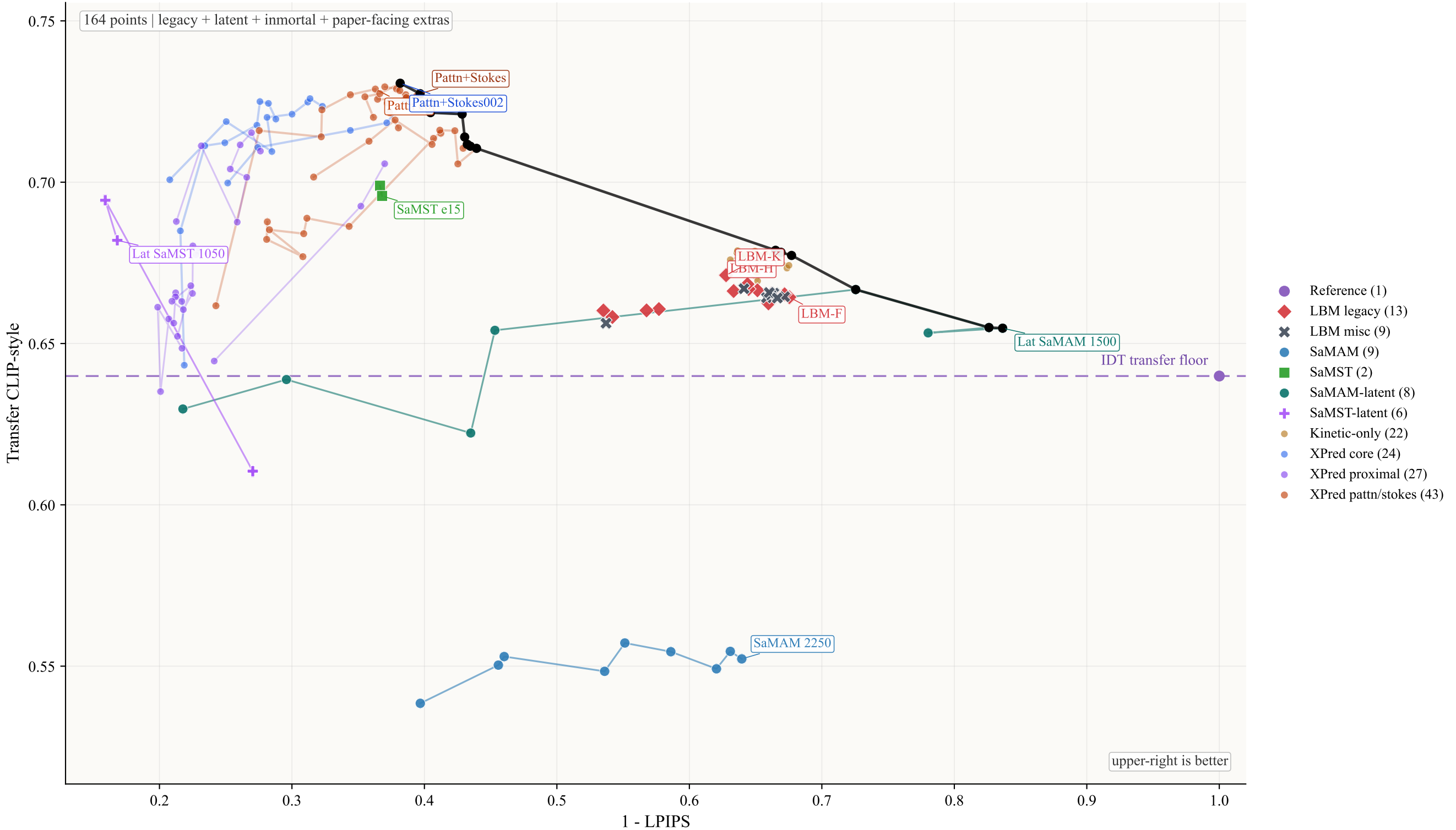
Distinct5-512 transfer landscape with all recorded operating points
