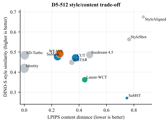
Fig. S3. D5-512 style/content plane. WEAVE is not the maximum-style point but lies in the low-LPIPS region among methods that clear the IDT style reference.
