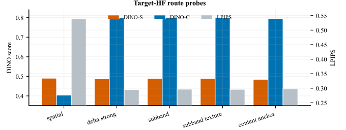
Fig. S2. Target-HF route probes. Spatial injection raises style but collapses content; pooled subband routes keep content at nearly the same style level.
