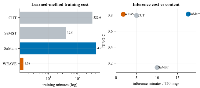
Fig. S4. Training minutes (left, log scale) and inference minutes versus DINO-C (right) for the learned methods.
