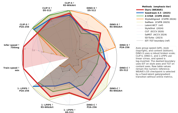
Figure 5: Style, content, and cost across three benchmarks. The dashed boundary uses IDT on style axes and TGT on content axes. DINO-S uses a broken visual scale; other metric axes are linearly normalized and speed axes are log-inverted. The D5 point uses the oriented-HF route selected by internal dynamics; Table 1 gives raw values.
