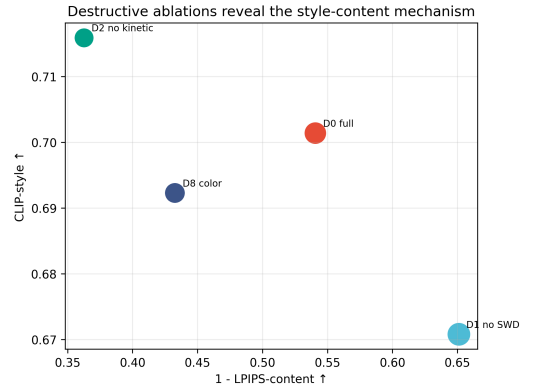
Figure 5: Destructive ablations. Removing terminal SWD improves content but weakens style, while removing kinetic regularization increases style at the cost of severe content degradation.
