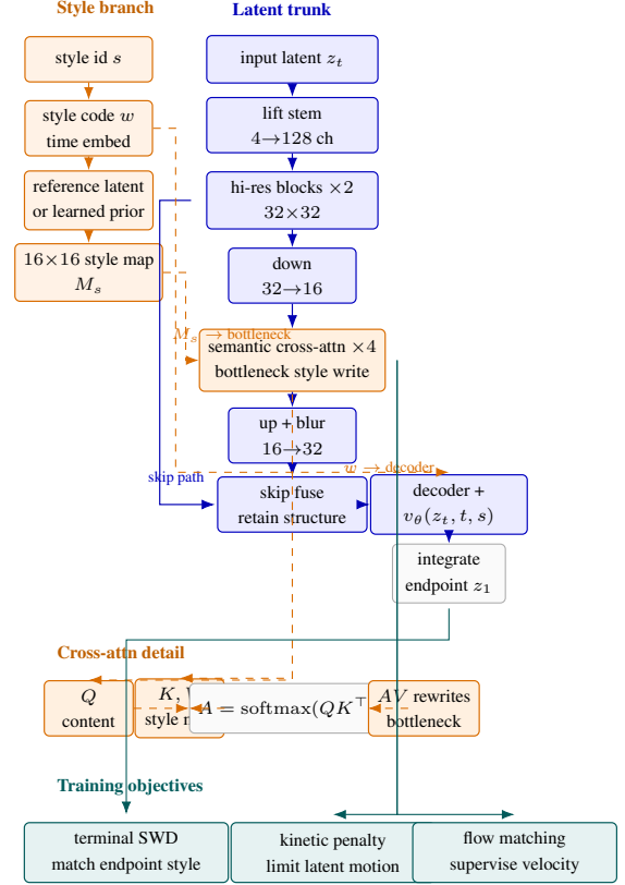
Figure 1: Overview of the latent transport model.
