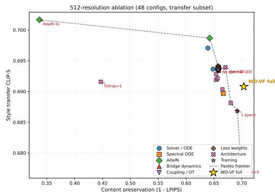
Figure 3: 512-resolution ablation scatter plot. Each point is one of 48 ablation configurations, colored by theoretical axis; the gold star marks the full WD-VF model. The dashed line is the Pareto frontier in the CLIP-S vs. 1-LPIPS plane. Three destructive clusters (AdaIN 4 \times , extrapolation 1, and LR 10 \times ) fall clearly off-frontier, validating the theoretical predictions.
