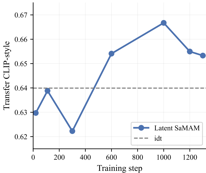
(a) Style vs. idt
