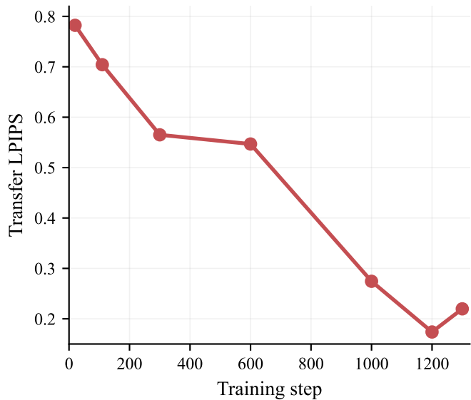
(b) Content distance
