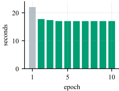
Epoch time
