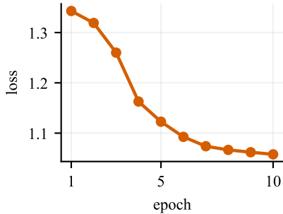
Training loss
