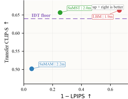
Figure 3: Matched same-cost Distinct5-512: transfer CLIP-S vs. 1 - LPIPS with the transfer-only IDT floor.
