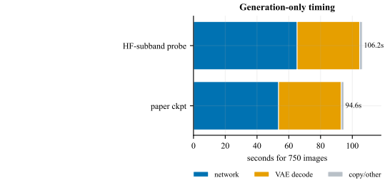
Figure 5: Generation-only timing decomposition on a single RTX 3060 (12 GB). VAE decode is a large fixed cost; the compact velocity network remains the dominant method-specific component.
