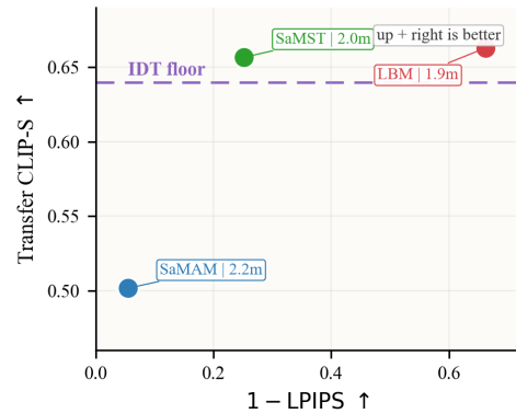
Figure 3: Matched same-cost Distinct5-512 view: transfer CLIP-S vs. 1 - LPIPS with the transfer-only IDT floor.
