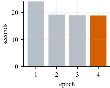
Epoch time
