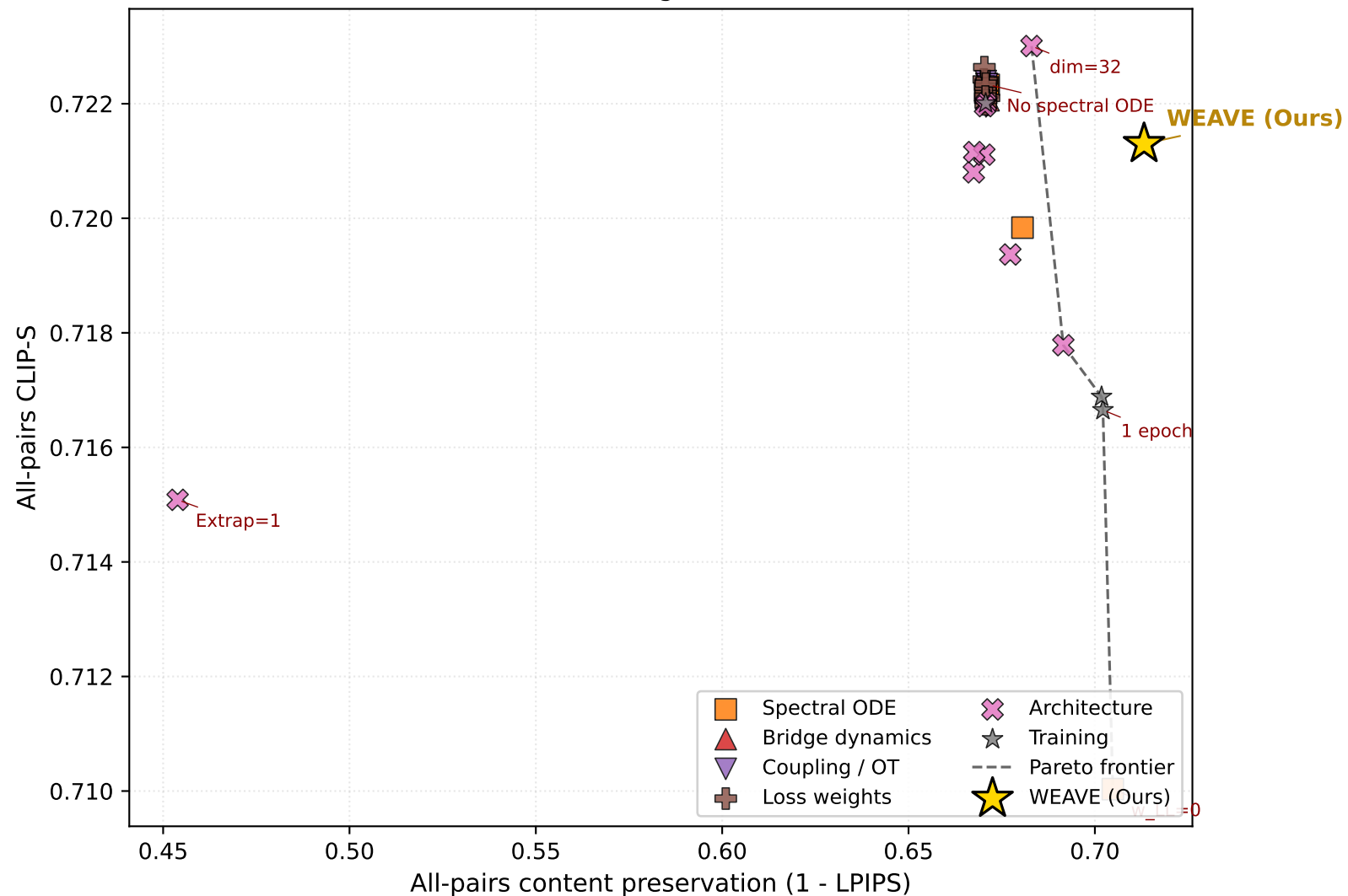
512-resolution ablation (38 configs, AdaIN & Solver axes omitted)
