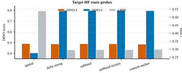
Figure 9: Mechanism-probe comparison. Spatial target-HF injection raises style but collapses content, while pooled/subband target-HF routes preserve content at nearly the same style level. prior but cannot replace the image-specific HF route.
