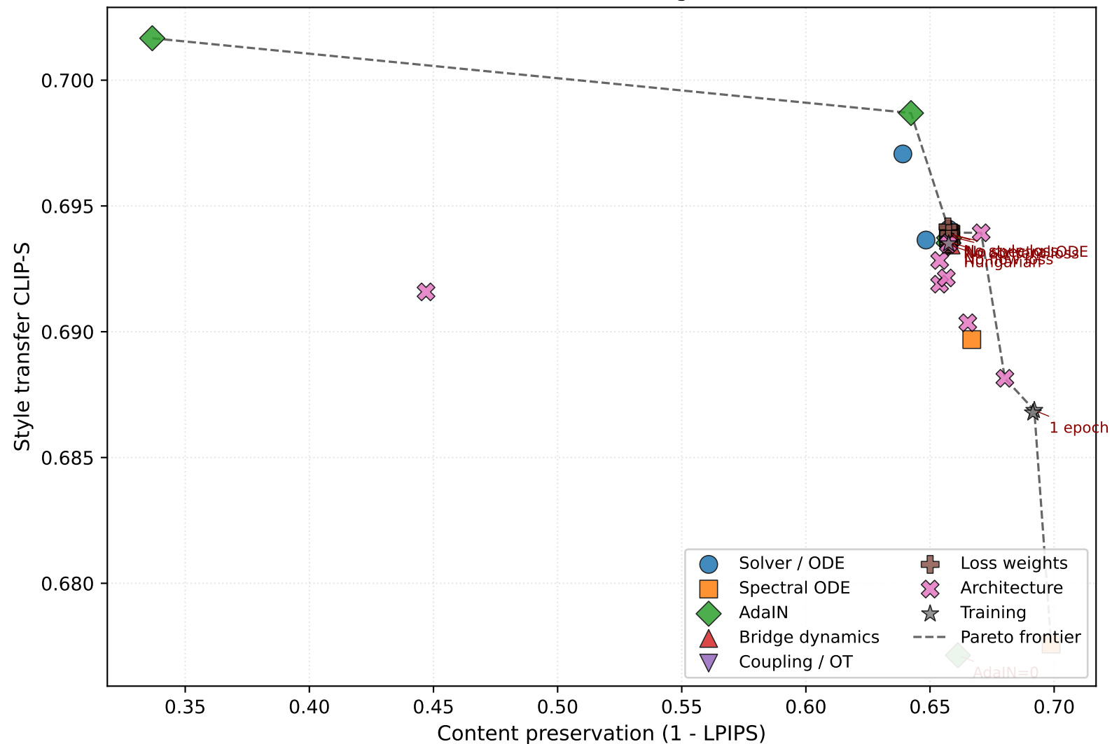
512-resolution ablation (48 configs, transfer subset)
