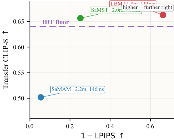
Figure 3: Matched-budget Distinct5-512 same-cost performance plot. Higher and further right is better: transfer CLIP-S is plotted against 1 - \text{LPIPS} , and the dashed line marks the transfer-only IDT floor. Under roughly two-minute training budgets, LBM stays in the favorable upper-right positive-IDT region, same-cost SaMST sits only slightly above IDT at much larger displacement, and same-cost SaMAM remains below IDT.
