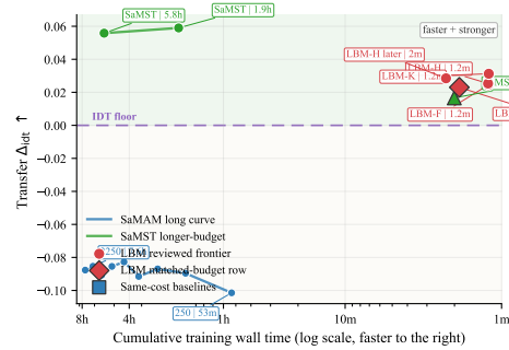
Figure 6: Evidence-closed Distinct5 timing records plotted as transfer-only \Delta_{\text{idt}} against cumulative training wall time under the reproduced full 5 \times 5 / 750-output protocol. The horizontal axis is log-scaled and inverted so faster adaptation appears to the right. LBM is shown in two roles: the retained reviewed frontier points around 1.2 minutes and the later step-350 matched-budget rerun. SaMAM is shown both as the exact same-cost row and as bounded pre-2250 timing records with the active manuscript boundary fixed at the trusted 2250 checkpoint; SaMST is shown both as the exact same-cost row and as the longer retained operating point. The plot therefore preserves the calibration between the retained frontier and the matched-budget rerun rather than serving as a closed normalized time-to-parity claim.
