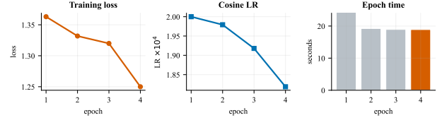
Figure 4: Training dynamics for the selected D5-512 checkpoint. Training stops at epoch 4 when the high-frequency conditioning gates increase and the shared LL/HF gradient ratio contracts sharply relative to the preceding epoch.
