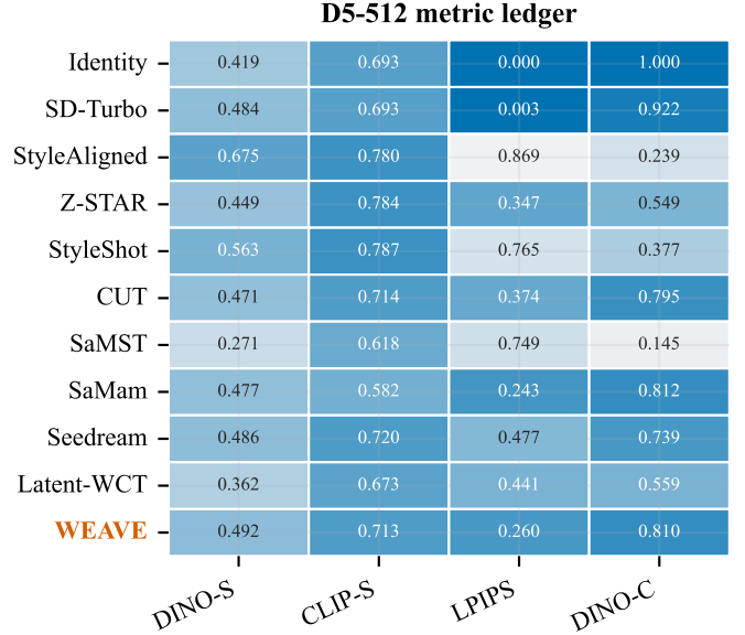
Figure 6: D5-512 metric ledger as a heatmap. LPIPS cells are color-normalized after inversion for readability, while annotations show raw values.
