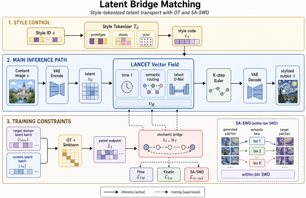
Figure 1: Overview of Latent Bridge Matching. The style tokenizer produces style-side controls from the target style identifier, and the LANCET vector field executes those controls as latent transport. Target-domain latents enter only through training-side OT endpoint construction and SA-SWD terminal matching; they are not inference-time conditioning inputs. Solid arrows denote the active inference path and dashed arrows denote supervision.
