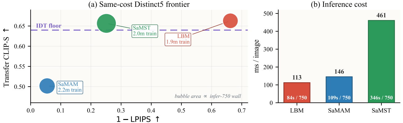
Figure 1: IDT-calibrated same-cost Distinct5-512 summary under the shared full 5 \times 5 / 750 -output packet. In (a), higher and further right is better: transfer CLIP-S is plotted against 1 - \text{LPIPS} , the dashed line marks the transfer-only IDT floor, and bubble area denotes infer-750 wall time. The LBM point shown here is the explicit matched-budget step-350 packet used for the page-1 comparison, not the strongest retained LBM frontier point. Under matched roughly two-minute training budgets, that packet still occupies the favorable region, same-cost SaMST stays only slightly above IDT at much larger displacement, and same-cost SaMAM remains below IDT. In (b), direct inference cost shows that the same-cost SaMST point is also the slowest executor.
