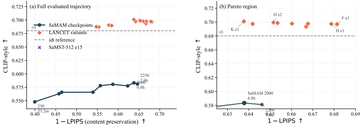
Figure 5: Distinct5-512 style-content frontier. Panel (a) shows the full evaluated trajectory and operating-point cloud under the reproduced 5 \times 5 / 750 -output protocol. Panel (b) zooms into the frontier region used for direct LBM-vs-baseline operating-point comparison; it is not a separate metric or filtered evaluation set. The dashed horizontal line marks the idt no-op CLIP-style level. LBM points are the best tokenizer-queue variants, the SaMAM curve shows cumulative training progress, and the SaMST-512 point marks a high-style, high-damage regime.
