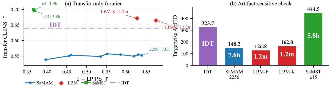
Figure 1: IDT-calibrated Distinct5-512 transfer-only results: SaMAM edits without beating IDT, SaMST beats IDT with large displacement and high ArtFID, and LBM-F/K beat IDT in a lower-damage region.
