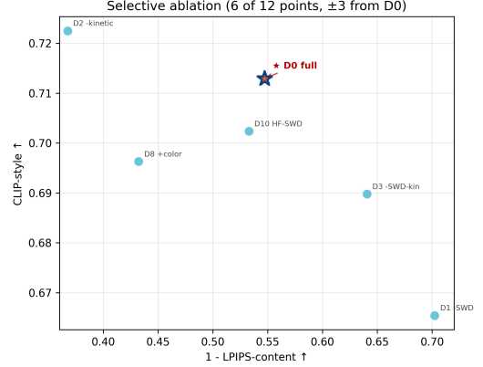
Figure 5: Destructive ablations. Removing SA-SWD improves content but weakens style, while removing kinetic regularization increases style at the cost of severe content degradation.
