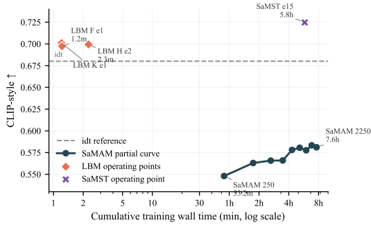
Figure 7: Same-scope Distinct5 timing-context artifact under the reproduced full 5 \times 5 / 750-output protocol, with cumulative training wall time and evaluation excluded from the horizontal axis. LBM is shown as reviewed operating-point records, SaMAM as the currently indexed partial curve, SaMST as the currently available operating point, and idt as the unchanged-image reference. This figure is used as bounded timing context rather than as a closed normalized time-to-parity claim.
