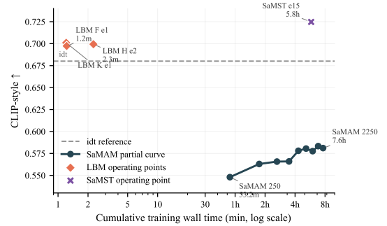
Figure 4: Same-scope Distinct5 timing-context artifact under the reproduced full 5 \times 5 / 750-output protocol, with cumulative training wall time and evaluation excluded from the horizontal axis. LBM is shown as reviewed operating-point records, SaMAM as bounded pre-2250 timing records with the active manuscript boundary fixed at the trusted 2250 checkpoint, SaMST as the currently available operating point, and idt as the unchanged-image reference. This figure is used as bounded timing context rather than as a closed normalized time-to-parity claim.
