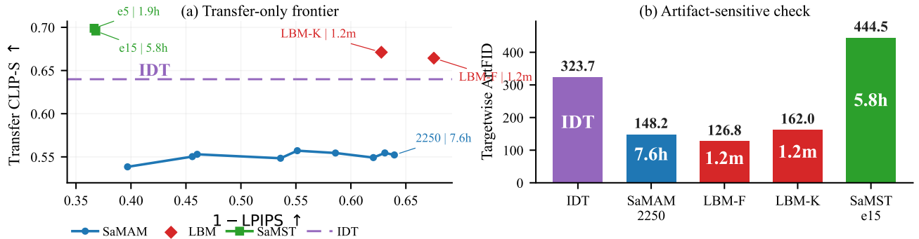
Figure 1: IDT-calibrated Distinct5-512 transfer-only operating points. LBM-F/K are the lowest-damage reproduced points above IDT; SaMST reaches higher raw style only in a high-displacement, high-targetwise-ArtFID region, and the validated SaMAM run remains below IDT.
