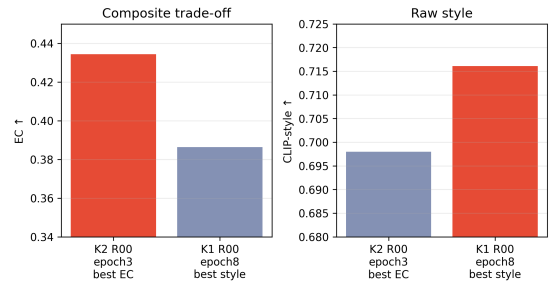
Figure 4: Summary of the 40-run category-weight sweep. K2 balanced default gives the best EC, whereas K1 balanced default gives the best raw CLIP-style among evaluated checkpoints.
