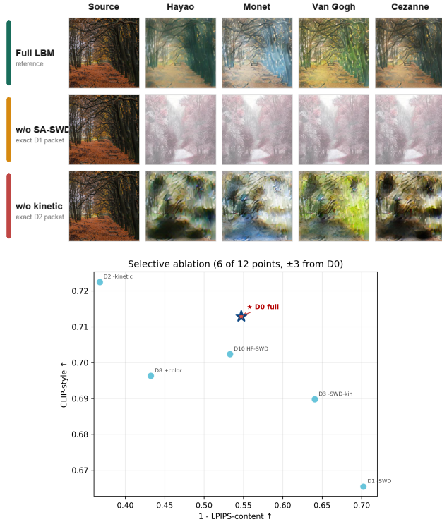
Figure 4: Mechanism ablations on the historical standard benchmark. Top: aligned photo-to-art directions for one shared source image and four target domains. The Full LBM row uses the retained standard-benchmark model as a clean reference for that source image, while the lower two rows are the exact archived D1 and D2 destructive packets. Removing SA-SWD leaves pale near-identity outputs with weak target-style commitment, whereas removing kinetic regularization amplifies texture at the cost of broken geometry, color spill, and unstable local structure. Bottom: the corresponding CLIP-S / LPIPS frontier from the destructive-ablation packet.
